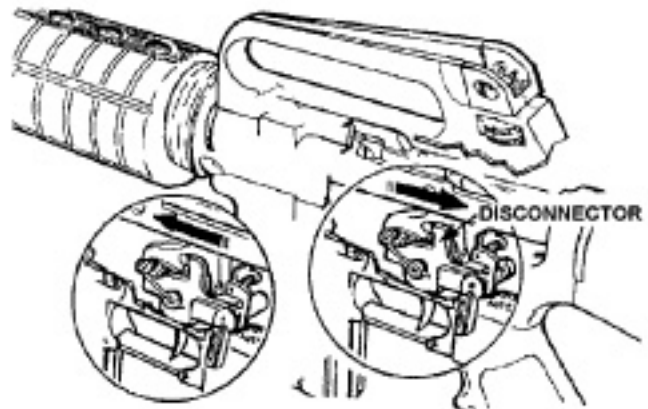
Figure 2-10. Cocking.
